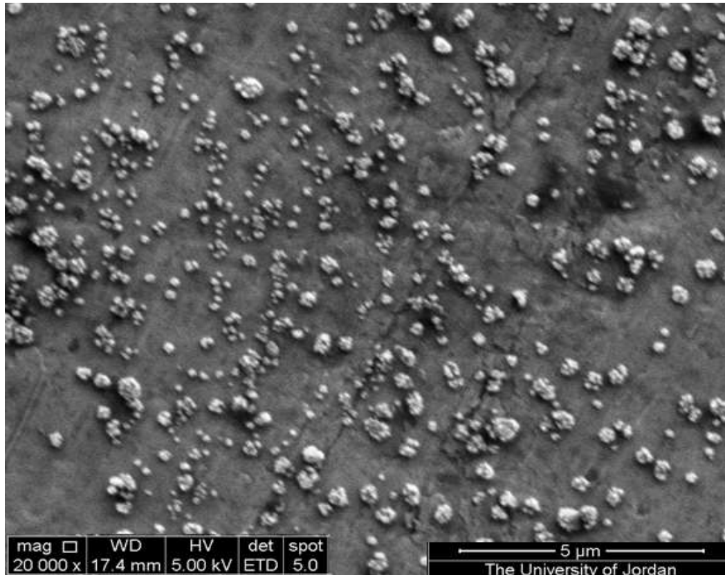
Fig.1 SEM Image of Platinum Nanoelectrode Coated on Tantalum Substrate
