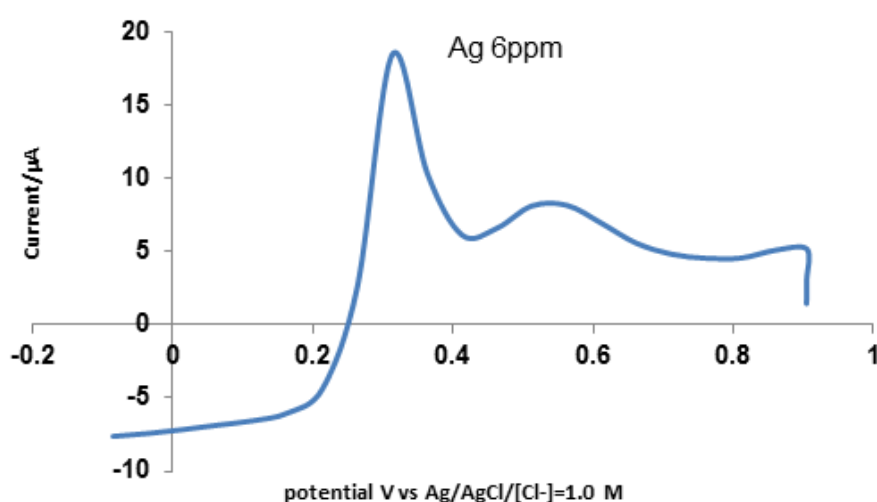
Fig.5 Cyclic voltammograms of \text{Ag}^{2+} solutions with 6 ppm concentration using the Platinum nanoelectrode at a scan rate of 50 \text{ mV s}^{-1} .
