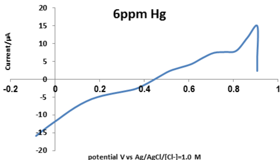
Fig.4 Cyclic Voltammograms of \text{Hg}^{2+} Solutions with 6 ppm Concentration using the Platinum Nanoelectrode at a scan rate of 50 \text{ mV s}^{-1} .
