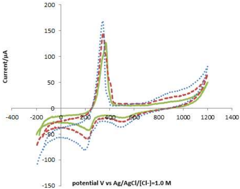
Fig.7 OSWVs of 2.5 M Ag 2 + Ammonium Acetate Solution using the Platinum Nanoelectrode with different days.
