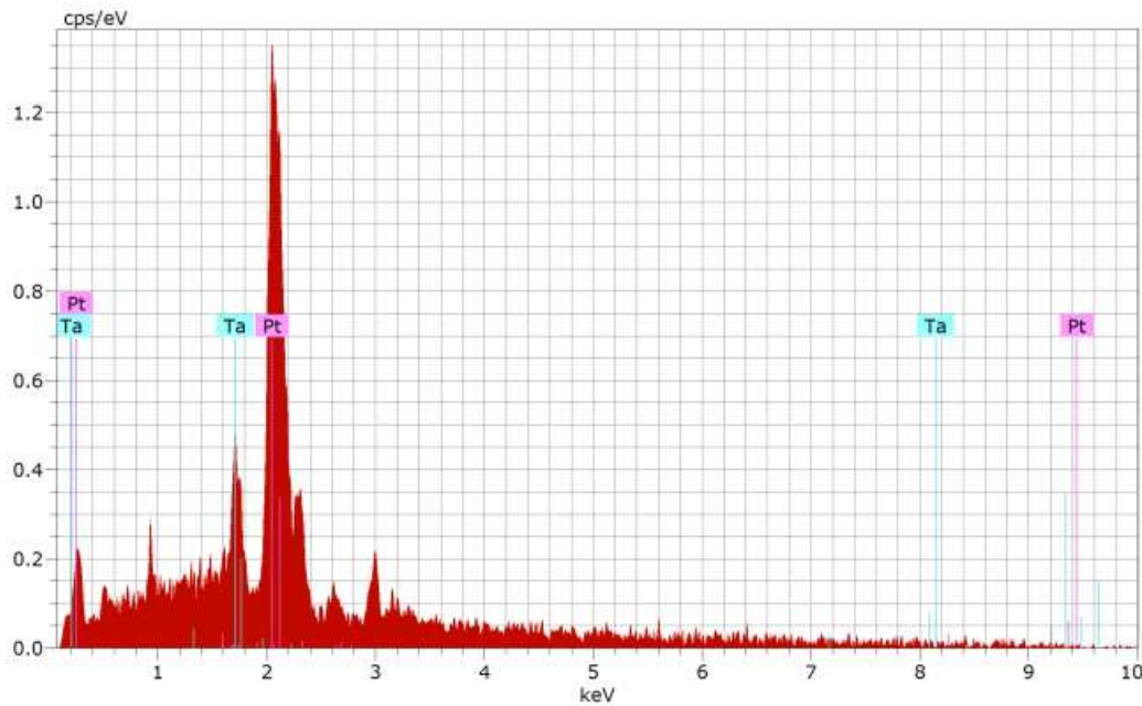
Fig.2 EDX Image of Platinum Nanoelectrode Coated on Tantalum Substrate
