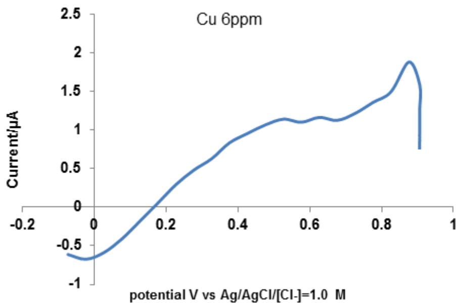
Fig.3 Cyclic Voltammograms of \text{Cu}^{2+} solutions with 6 ppm concentration using the Platinum Nanoelectrode at a scan rate of 50 \text{ mV s}^{-1} .
